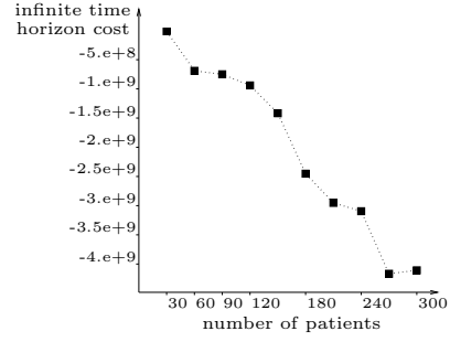
Figure 4. Influence of the number of patients participating to the clinical trials on the infinite horizon cost corresponding to the computed STI strategies. Data generation follows the protocol described in Section 3.2. To compute the infinite horizon cost associated to a given number of patients, we run RL on the trajectories generated by these patients and estimate J^{\hat{\mu}_{400}}(x) obtained when a patient initially in the “non-healthy” steady-state is treated by the learned strategy ( J^{\hat{\mu}_{400}}(x) = \sum_{t=0}^{\infty} \gamma^t c(x_t, \hat{\mu}_{400}^*(x_t)) with x = (T_{1_0}, T_{2_0}, T_{1_0}^*, T_{2_0}^*, E_0, V_0) = (163573, 5, 11945, 46, 63919, 24) ).
