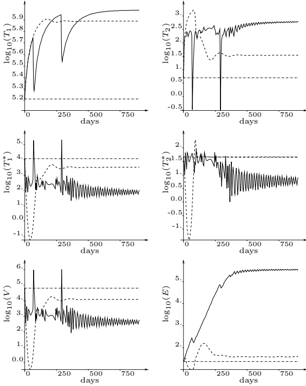
Figure 2. The curves represent the time evolution of the different cells count ( T_1 , T_2 , T_1^* , T_2^* ), of the number of free virus particles ( V ) and of the number of immune effectors ( E ) for a patient being treated from “non-healthy” steady-state. The solid curve (—) corresponds to the STI strategy plotted on Fig. 3 and computed by the reinforcement learning algorithms. The dashed curves (---) represent the time evolution of these variables when there is no interruption in the treatment (i.e. \epsilon_{1t} = 0.7 and \epsilon_{2t} = 0.3 , \forall t \geq 0 ) and the dotted curves (-·-) represent their time evolution when there is no treatment (i.e. \epsilon_{1t} = \epsilon_{2t} = 0 , \forall t \geq 0 ).
