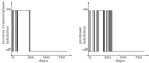
Figure 3. Representation of the STI treatment for a patient treated from early stage of infection. The STI treatment is computed by the reinforcement learning algorithms on clinical data generated by 300 patients.
